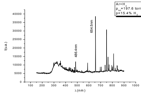
Figure 6 Emission spectrum of a DC discharge in (Ar+15.4 %H 2 ) at p_{\text{tot}}=197 Torr.
