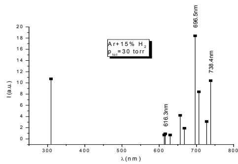
Fig. 4 – Emission spectrum of a PDP-type discharge in (Ar+15 % H 2 ).
