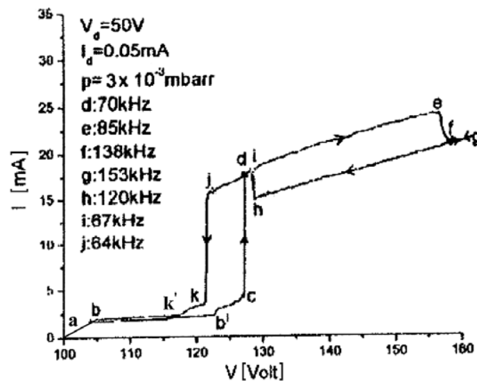
Fig. 1 – Static I(V) characteristic obtained from a plasma diode. Gas argon, V_d voltage I_d current of the plasma source. Most of the voltage V is supported by the plasma column.
