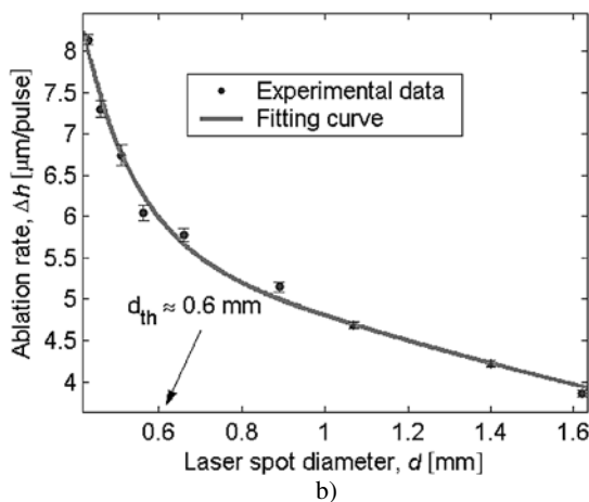
Fig. 2 – Ablation rate of aluminum as a function of the laser spot diameter. The laser wavelength is 1064 nm in panel (a), and 532 nm in panel (b).
