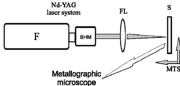
Fig. 1 – Experimental setup: F – laser head generating the fundamental wave, SHM – second harmonic generator module, FL – focusing lens, MTS – mechanical translation stage.
