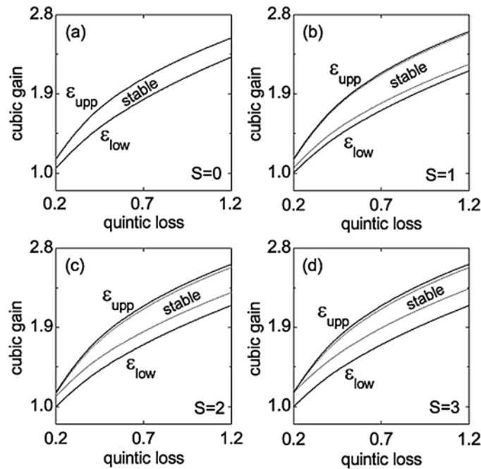
Fig. 5 – The existence and stability domains of 3D dissipative solitons, with S = 0, 1, 2, 3 , for \beta = 0.5 , in the plane of the quintic-loss and cubic-gain coefficients, (\mu, \varepsilon) .
