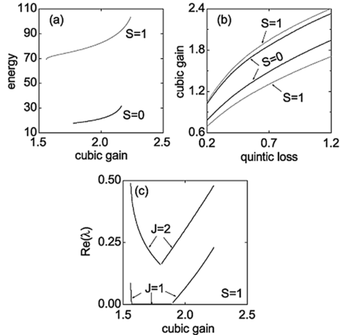
Fig. 6 – (a) The energy of fundamental ( S=0 ) and vortex ( S=1 ) 3D dissipative solitons versus the nonlinear-gain parameter \varepsilon , for zero diffusivity, \beta=0 . (b) The existence and stability domains for these solutions. (c) The largest instability growth rate versus \varepsilon for the vortex solitons with S=1 .
