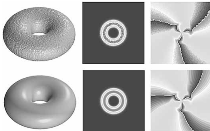
Fig. 8 – The recovery of a perturbed 3D vortex soliton with S = 3 , for \mu = 1 , \beta = 0.5 and \varepsilon = 2.3 . Upper row: the intensity ( |U|^2 ) and phase of the initial soliton perturbed by random noise. Lower row: The same in the self-cleaned soliton at z = 800 .
