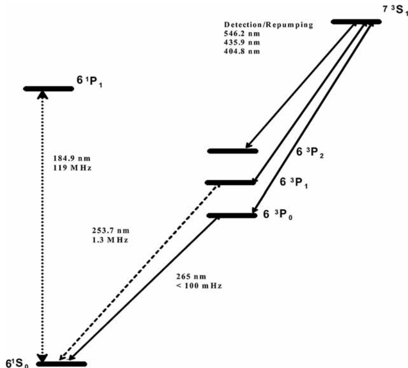
Fig. 1 – The lowest energy levels of mercury.
