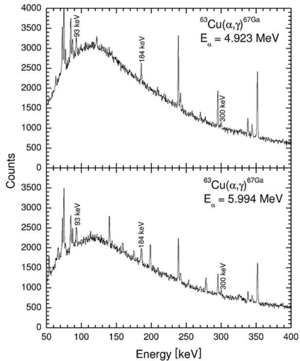
Fig. 1 – Partial HPGe \gamma -ray spectra of ^{67}\text{Ga} characteristic \gamma lines.
