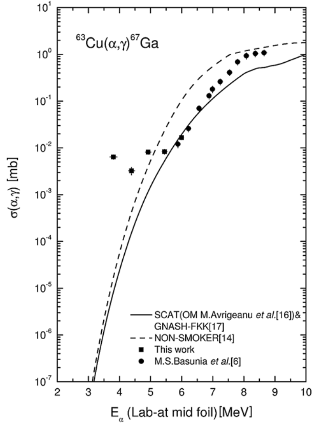
Fig. 2 – Comparison between experimental and theoretical cross section for the ^{63}\text{Cu}(\alpha, \gamma)^{67}\text{Ga} reaction (see text for details).
