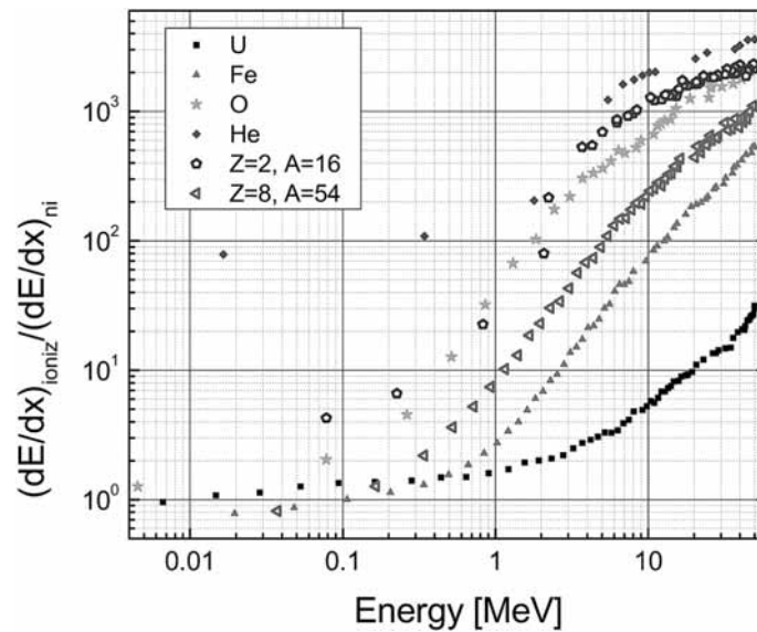
Fig. 1 – Ratio between ionizing and non-ionizing energy loss for ions of He, O, Fe, U, and for two hypothetical candidates for SQM.
