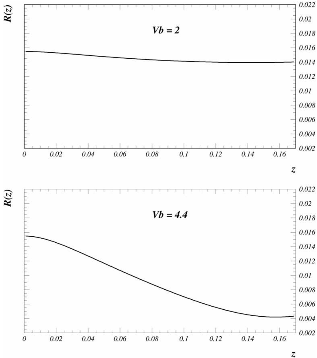
Fig. 2 – The solution R(z) of the paraxial equation for z \in [0, z_{m1}] .
