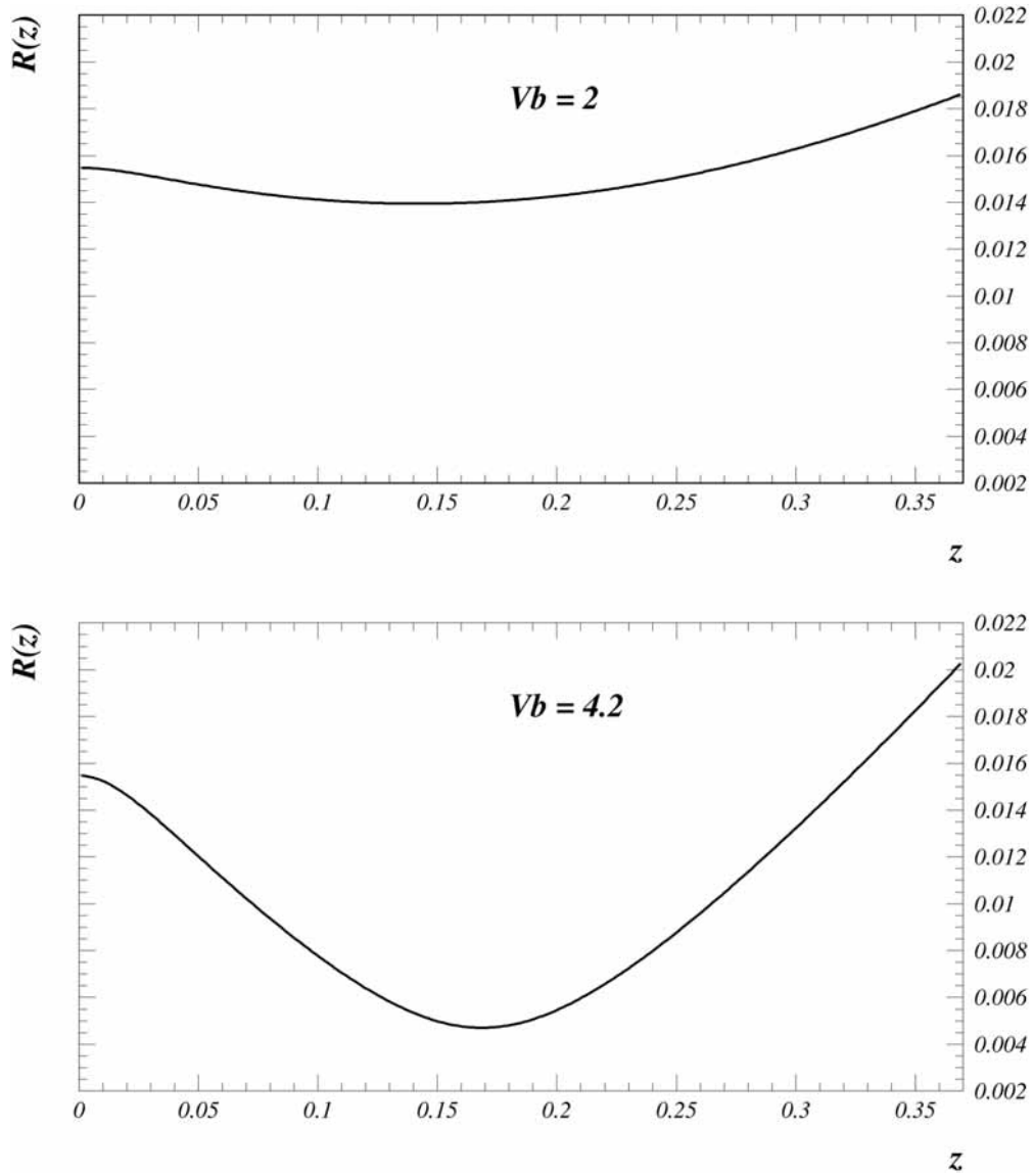
Fig. 3 – The solution R(z) of the paraxial equation for z \in [0, zm2] .
