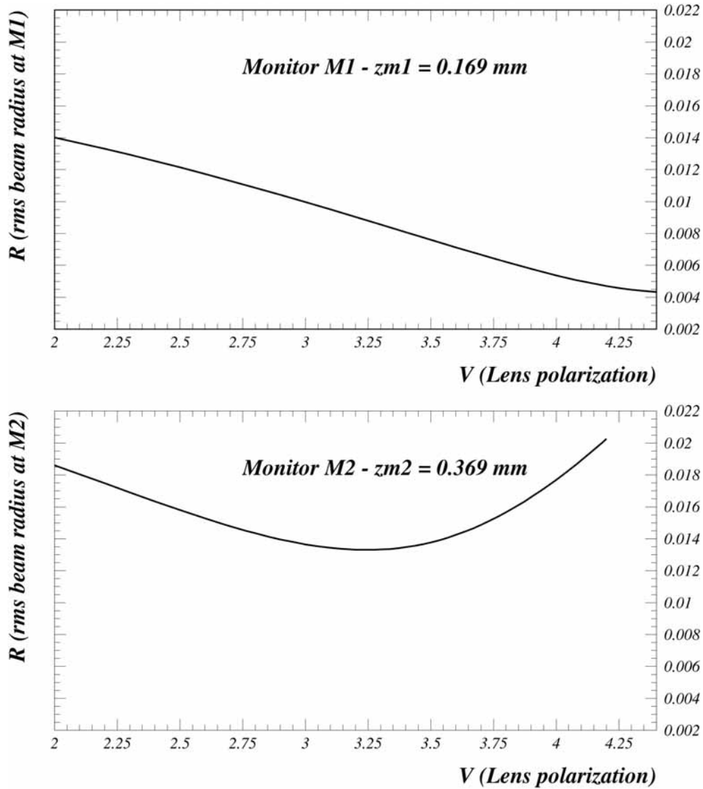
Fig. 1 – The root-mean-square beam radii ( R ) at the monitors in function of the lens polarization ( V ).
