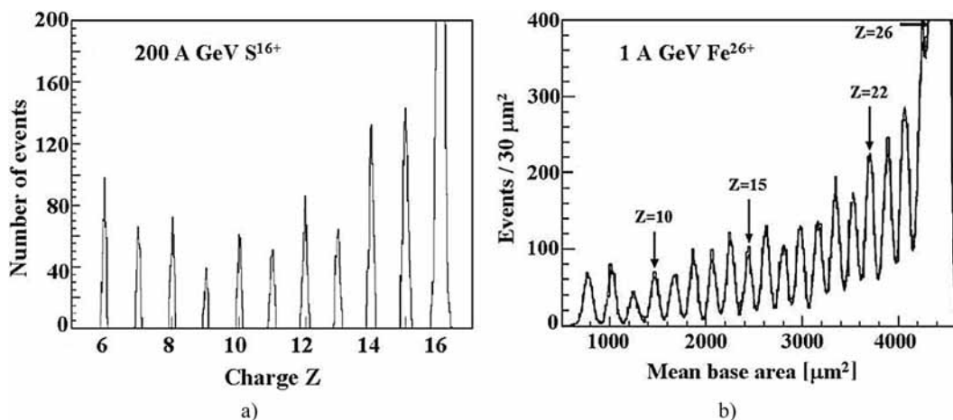
Fig. 6 – (a) Charge distribution of 200 GeV/nucleon \text{S}^{16+} ions and their fragments measured with CR39 NTDs (many measurements were made). (b) Charge distribution measured with CR39 detector sheets located after a \text{CH}_2 target exposed to 1 A GeV \text{Fe}^{26+} ions and their fragments.
