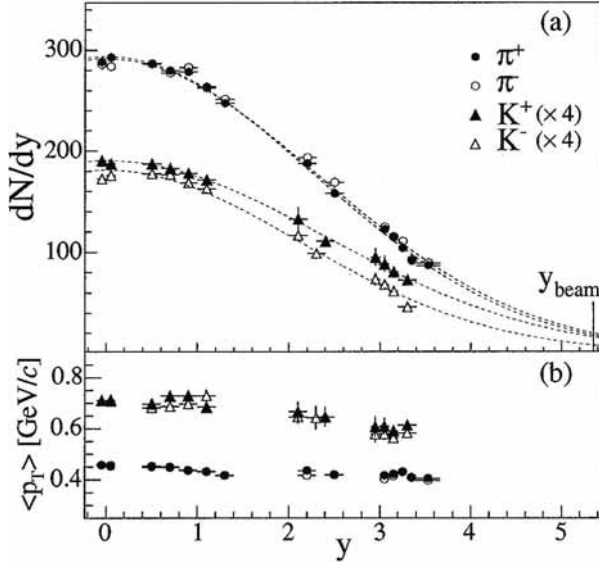
Fig. 8 – (a) Pion and kaon rapidity densities, dN/dy , and (b) their mean transverse momentum \langle p_t \rangle as a function of rapidity y . The kaon yields were multiplied by a factor of 4 for clarity. The dashed lines in (a) are Gaussian fits to the dN/dy distributions.
