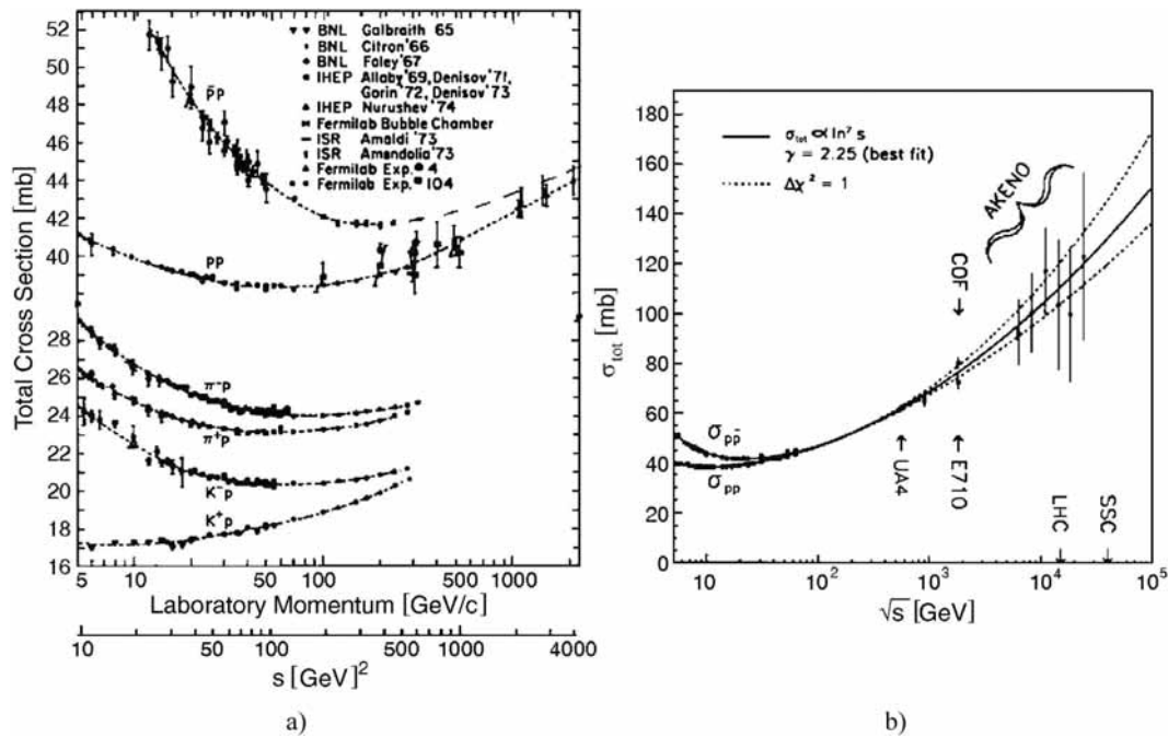
Fig. 1 – Compilation of total cross-sections (a) for high-energy hh scattering and (b) for higher energy \bar{p}p and pp , including cosmic ray measurements; the solid line is a Regge pole fit; the uncertainty in the energy trend is indicated by dashed lines.
