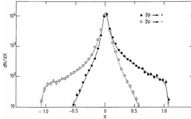
Fig. 4 – x -distributions of positive and negative particles produced \bar{p}p interactions at \sqrt{s} = 53 GeV [13]. Positive values of x correspond to the direction of the incoming protons. The slight differences between leading particles for x > 0 and x < 0 are due to the acceptance of the apparatus. The lines are only meant to guide the eye.
