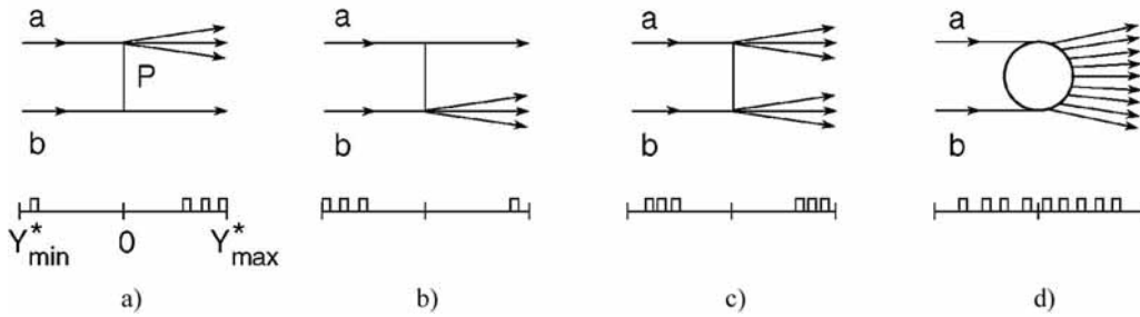
Fig. 2 – Pictorial description of inelastic, small p_t processes with characteristic rapidity distributions. P indicates Pomeron exchange. (a) Fragmentation of the beam particle a; (b) fragmentation of the target particle b; (c) double fragmentation of a and b; (d) inelastic non diffractive collisions.
