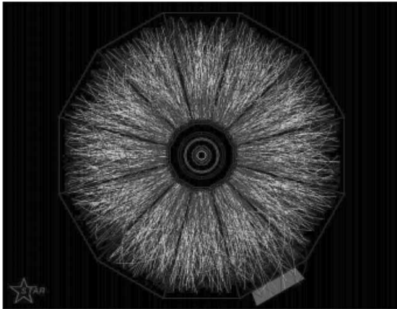
Fig. 7 – One of the first events recorded by the STAR detector at RHIC in the collision of two gold ions at \sqrt{s_{NN}} \sim 200 GeV/nucleon. The tracks indicate the paths of thousands of charged particles produced in the collision, as they pass through the STAR Time Projection Chamber.
