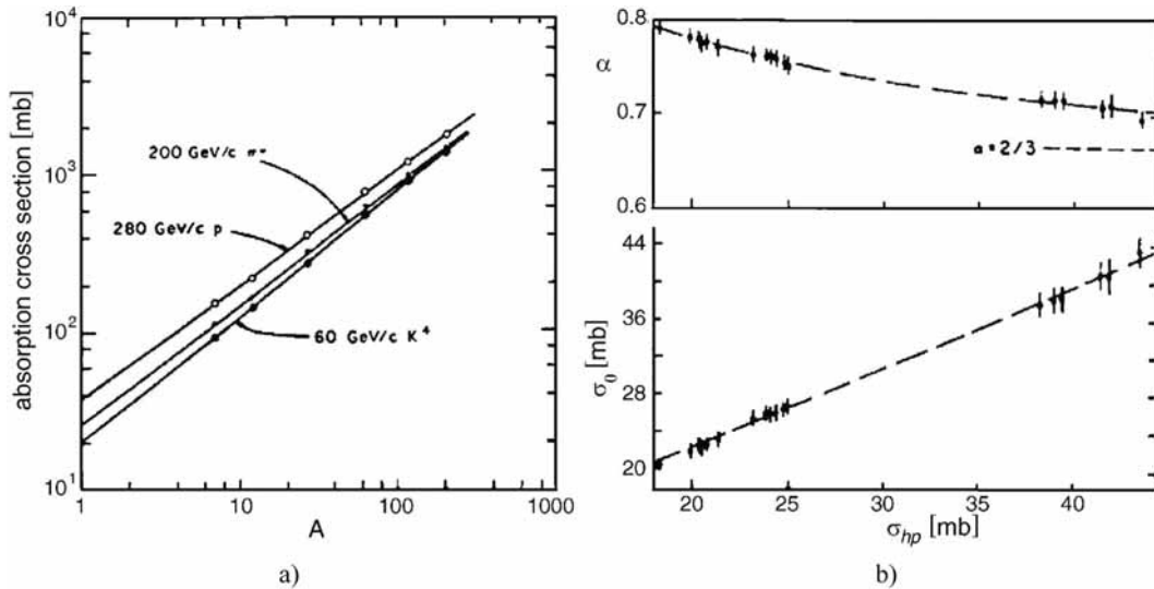
Fig. 5 – (a) Absorption cross-sections versus atomic weight A ; the solid lines are fits to eq. (3). (b) The parameters \sigma_0 and \alpha versus the corresponding hp total cross-section ( \sigma_{hp} ).
