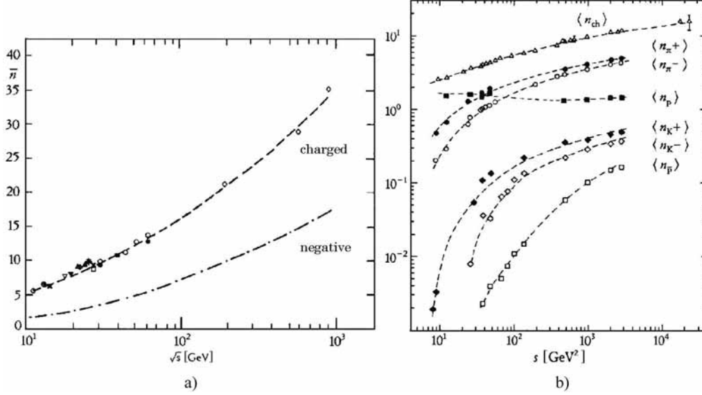
Fig. 3 – (a) Average charged multiplicities \bar{n} for \bar{p}p and pp collisions vs. E_{cm} = \sqrt{s} . (b) Average number of \pi^\pm , K^\pm , p and \bar{p} produced in pp collisions at the CERN ISR for c. m. energies up to 63 GeV.
