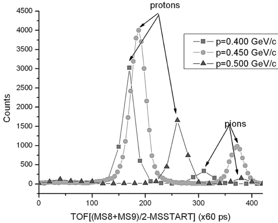
Fig. 4 – The TOF distributions of pions and protons for three modes of operation of the spectrometer.
