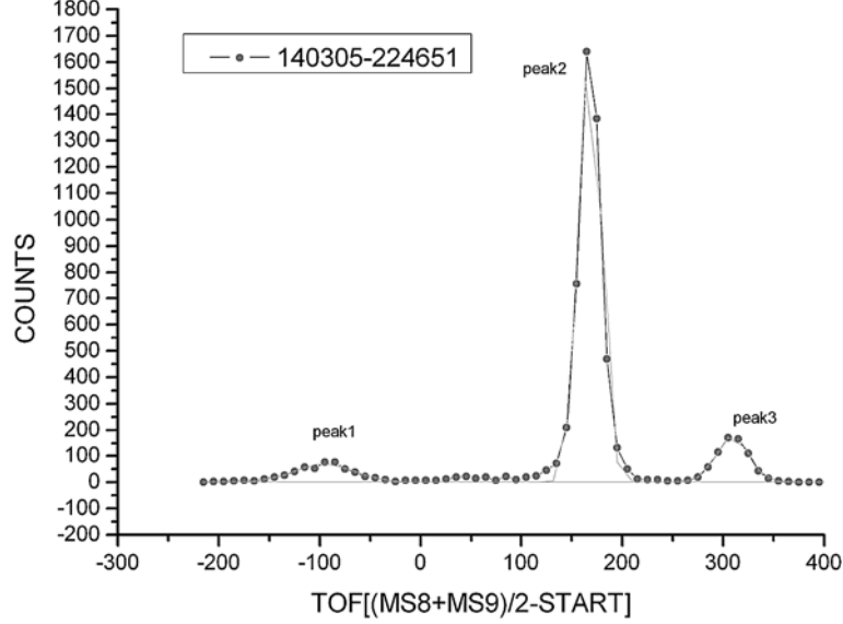
Fig. 3 – The TOF distribution of particles in the SP40 dipole magnet.
