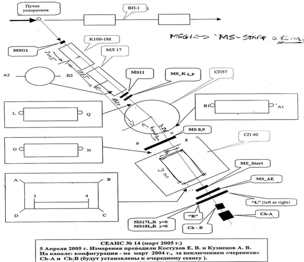
Fig. 2 – MARUSYA experimental set-up – the index of the silicon detectors.
