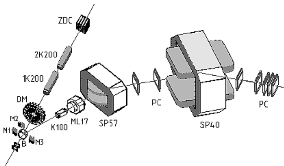
Fig. 1 – MARUSYA experimental set up – large view.
