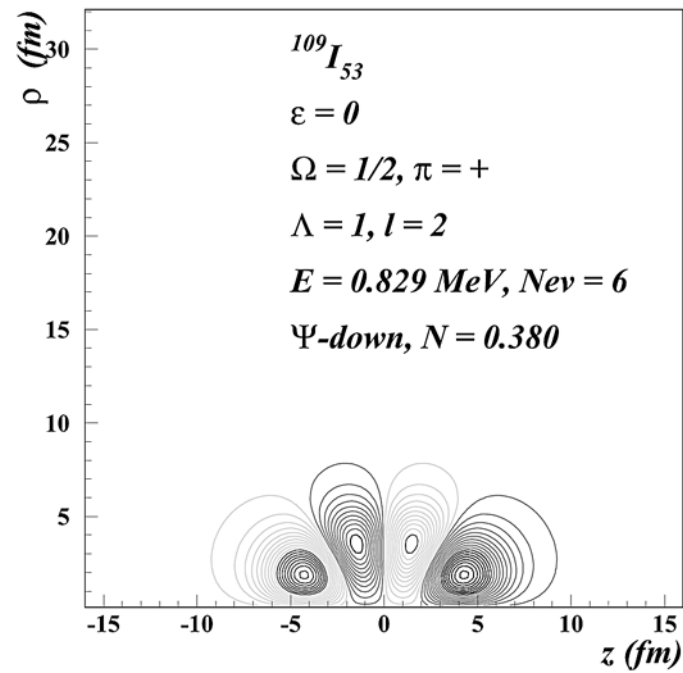
Fig. 3 – Initial w.f. – up and down (spherical).
