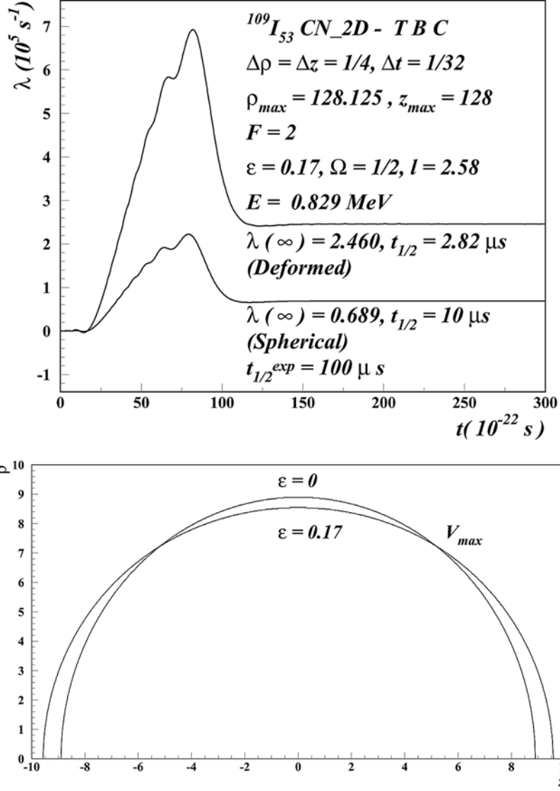
Fig. 6 – Decay rates – spherical + deformed and the top equipotential lines.
