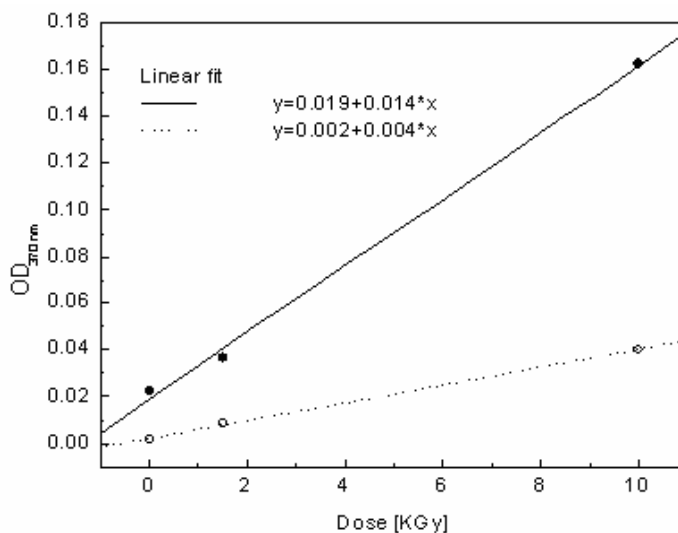
Fig. 2 – Dose dependence of the absorption at 370 nm of DNPH-carbonyl groups formed as a result of the radiolytic oxidation in the RAA samples: dilution 1/10 (●) and 1/100 (○) with 0.05 M phosphate buffer pH 7.5.
