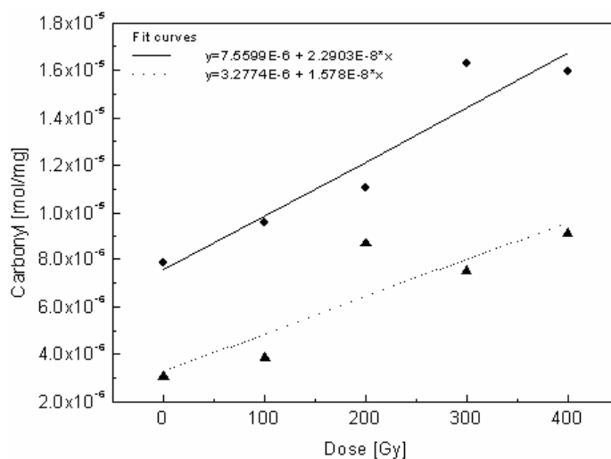
Fig. 1 – Dose dependence of the concentration of carbonyl groups formed as a result of the radiolytic oxidation of BSA in aqueous solution: 1.25 mg/ml BSA (▲) and 2.5 mg/ml BSA (●).
