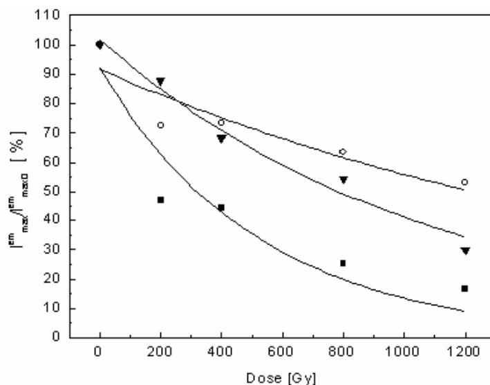
Fig. 3 – Relative fluorescence intensities and the corresponding fits as function of the irradiation dose, at three different testosterone-3-CMO-BSA concentrations: 1.25 mg/ml (■), 2.5 mg/ml (▼) and 5 mg/ml (○).
