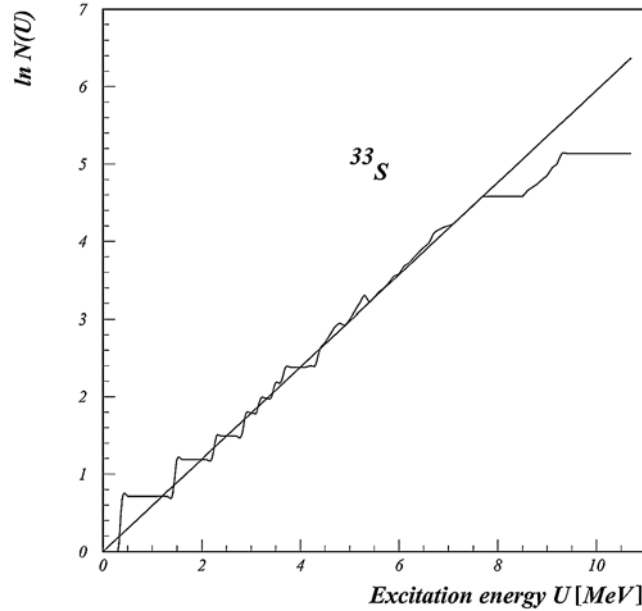
Fig. 1 – The cumulated histogram of discrete levels for ^{33}\text{S} in terms of the excitation energy U . The straight line represents the linear function from eq. (2.3) with U_0 = 0 and T = 1.68 MeV.
