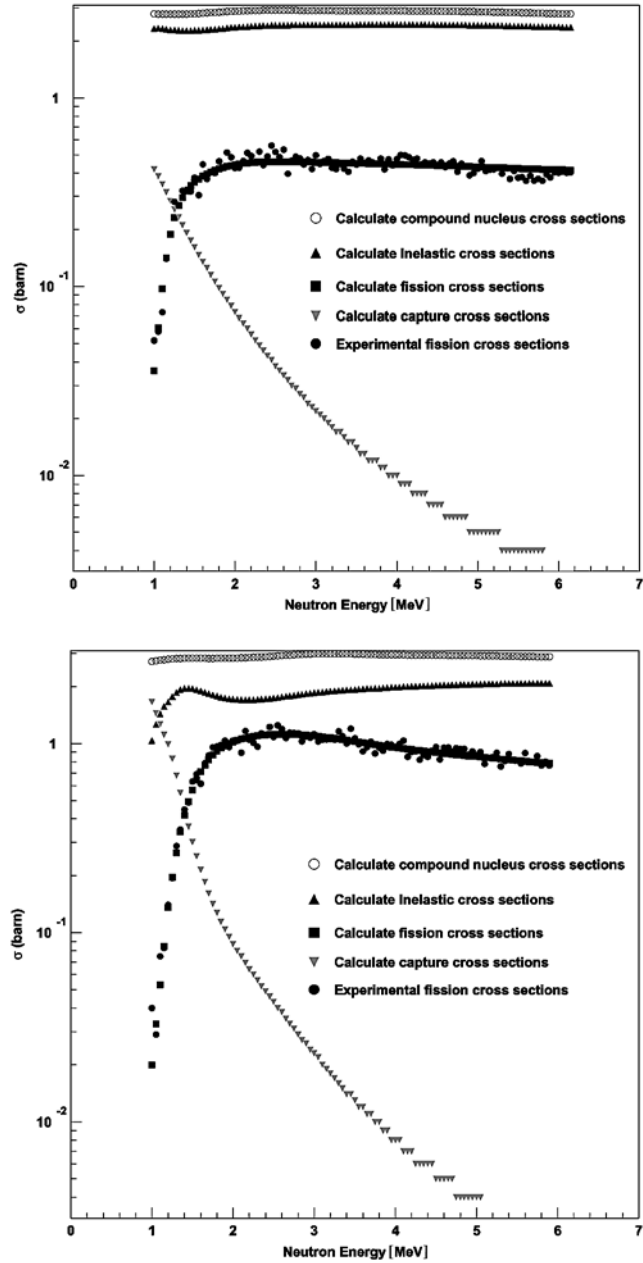
Fig. 6 – The comparison with experimental data of the fission cross sections for the neutron induced fission of ^{232}\text{Pa} together with the calculated capture, compound nucleus and inelastic cross sections (upper panel) and of ^{234}\text{Pa} (lower panel).
