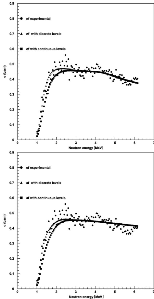
Fig. 4 – The comparison with experimental data of the cross sections for the neutron induced fission of ^{232}\text{Pa} calculated from the continuous densities given by the Ignatyuk method (upper panel) and by the modified Ignatyuk method (lower panel).
