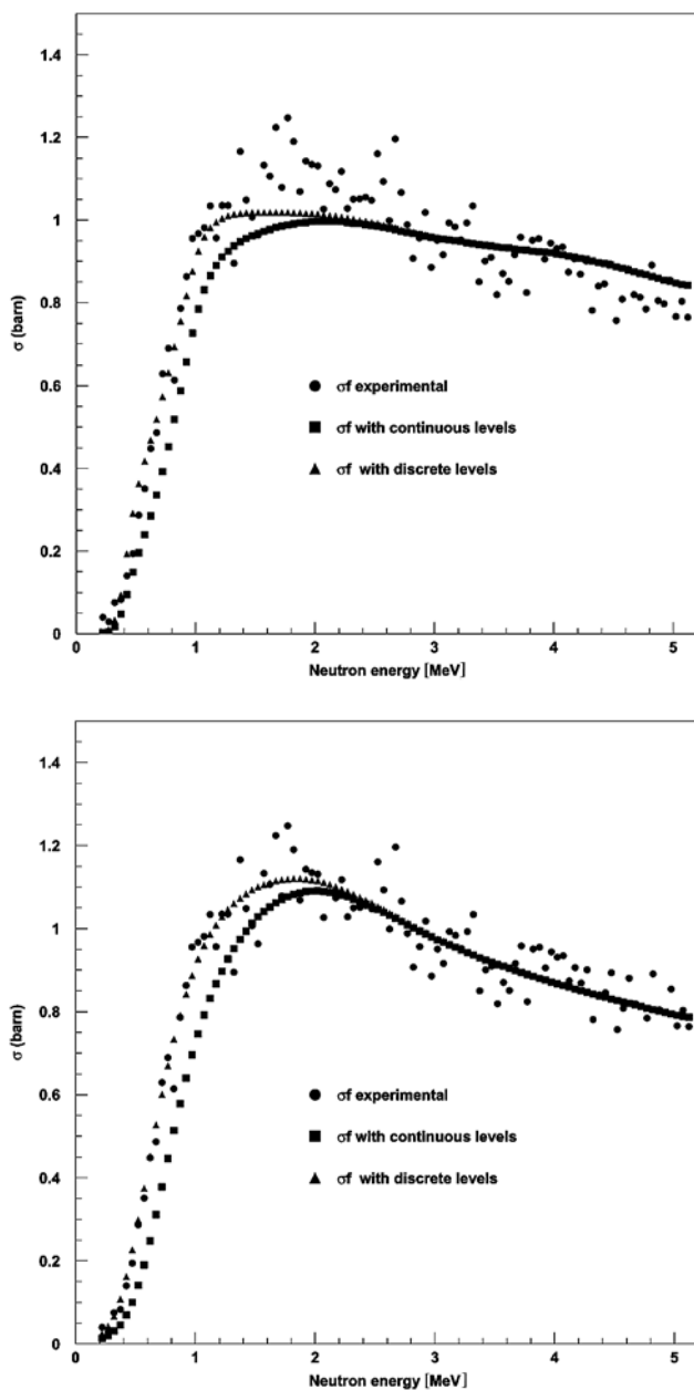
Fig. 5 – The comparison with experimental data of the cross sections for the neutron induced fission of ^{234}\text{Pa} calculated from the continuous densities given by the Ignatyuk method (upper panel) and by the modified Ignatyuk method (lower panel).
